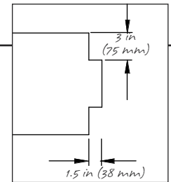
Figure 5: Post Spacer End Detail
