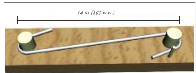
Figure 7: Stirrup Jig for Two-Course Bond Beam
