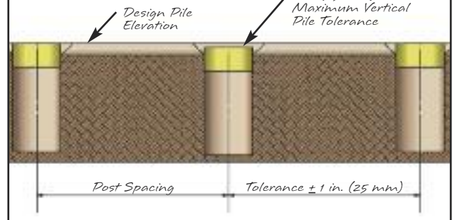
Level Piles
