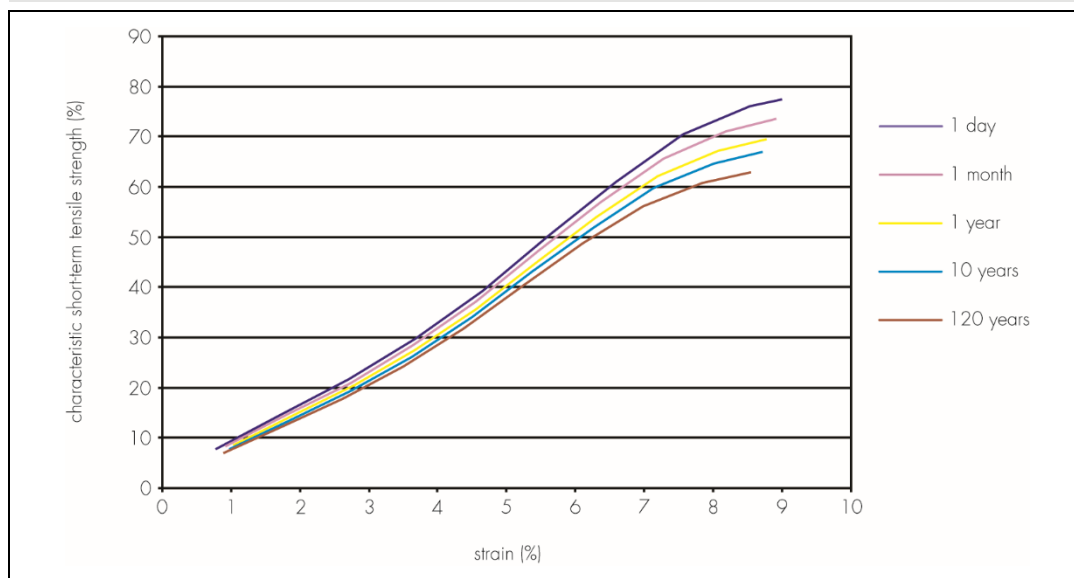
Figure 4 Isochronous curves for Fortrac T geogrids
